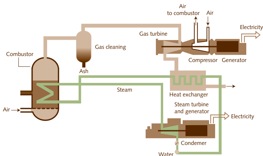
Pressurised fluidised bed. Combined cycle
